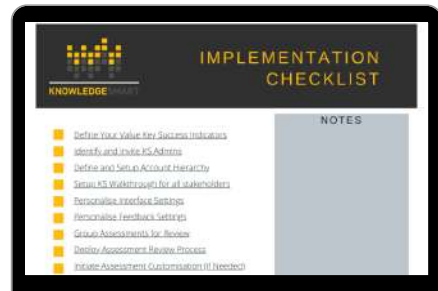
Implementation Checklist
